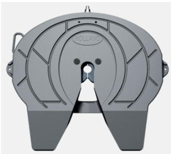
Obsolete (D=165kN) FW351 Fifth Wheel
