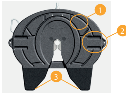
New Style FW351 Fifth Wheel (D=190kN)
