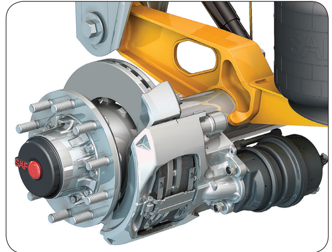
C88 Wheel End
