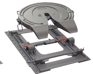
FW70 Top Plate Specification on SDS No-Tilt Base
