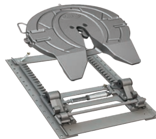
FW35 & FW33 Low Lube Top Plate Specification on ILS No-Tilt Base
