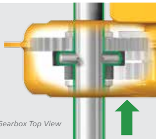
CRANKSHAFT ENGAGED IN LOW DRIVE GEAR
