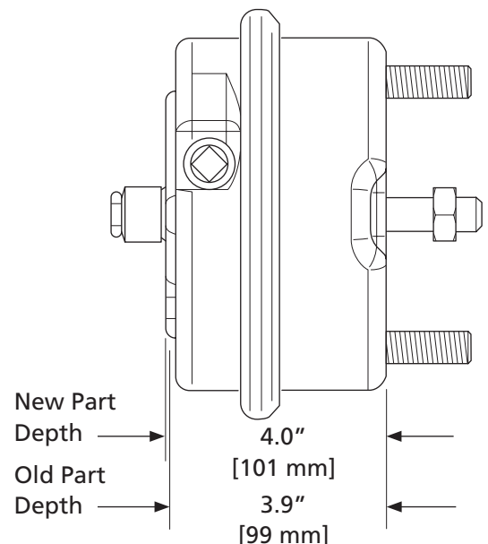
Air Chamber Dimensions
