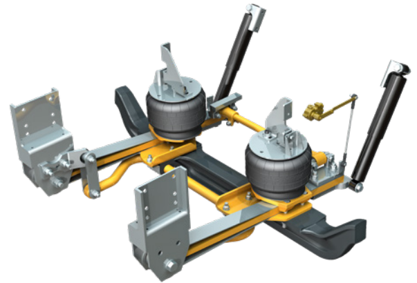
AS and ASB Front Steer Air Suspension Models
